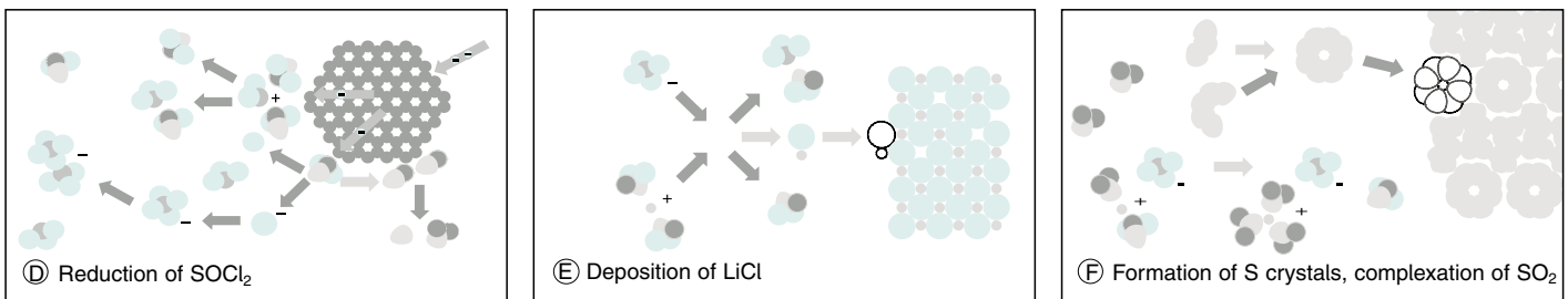
Figure 3-4 Reaction mechanism of lithium thionyl chloride batteries. The circles are enlarged views of the anode surface (lower left) and cathode surface (upper right). The anode surface is covered with the SEI (solid electrolyte interface) and the SPL (secondary porous layer) on top of it. On the cathode and on the separator, both lithium chloride and sulfur crystals have formed as reaction products.
