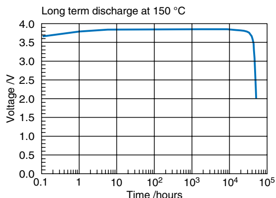
Figure 2-12 Long-term discharge of \frac{1}{2} AA size cells, type SL-550 at +150^{\circ}\text{C} for more than 5 years on a continuous load of 560\text{ k}\Omega corresponding to a current of 6\ \mu\text{A}
