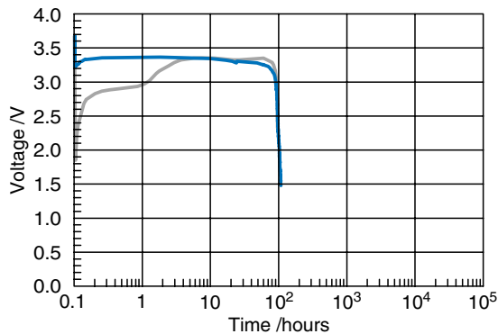
Figure 2-3 Discharge of \frac{1}{2} AA cells on 330 \Omega after one year of storage at +25 ^{\circ}\text{C} . Blue curve: SL-750 Grey curve: SL-350
