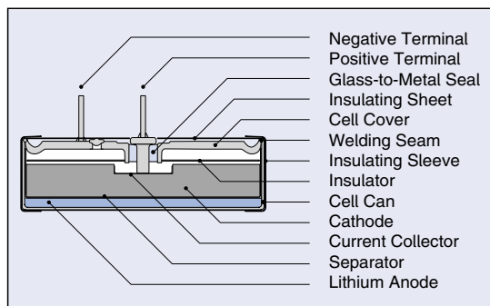
Figure 3-2 Cross sectional view of a 1/6D size cell (flat cell)
