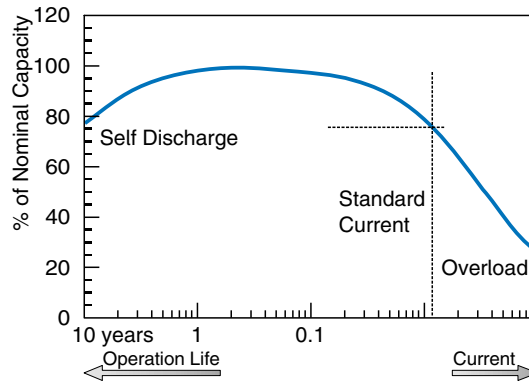
Figure 2-6 Dependence of capacity on current. Self discharge increases with operation life. Overload occurs if current exceeds the standard current corresponding to 76% of the saturation capacity.
