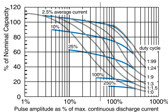
Figure 2-8 Effect of pulse discharge on available capacity to 2 Volts at 25°C grey curves: constant duty cycle blue curves: constant average current as % of nominal current Data obtained with SL-780 batteries
