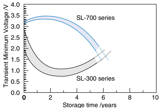
Figure 2-4 Typical behaviour of voltage delay over storage time for two basic series. Discharge at 25 ^{\circ}\text{C} using the 100 hour rate (2 \text{mA}/\text{cm}^2 ) Data obtained with \frac{1}{2} AA size on 330 \Omega
