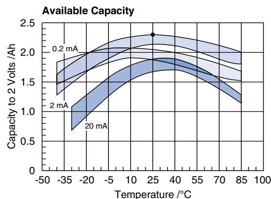
Figure 2-11 Temperature dependence of available capacity for three different current levels. Size AA, type SL-360
